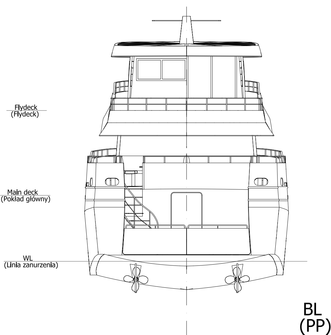
Stern view (Widok od rufy)
